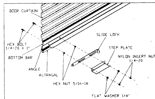
OPTIONAL BOTTOM BAR MOUNTED SLIDE LOCKS FIGURE 1
